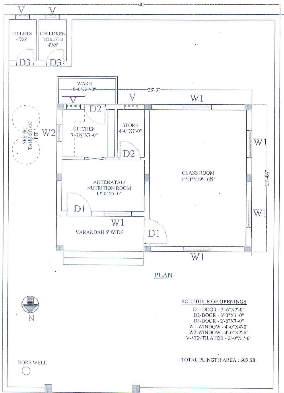
PLAN OF MODEL ANGANWADI BUILDING UNDER NREGS AND NABARD
