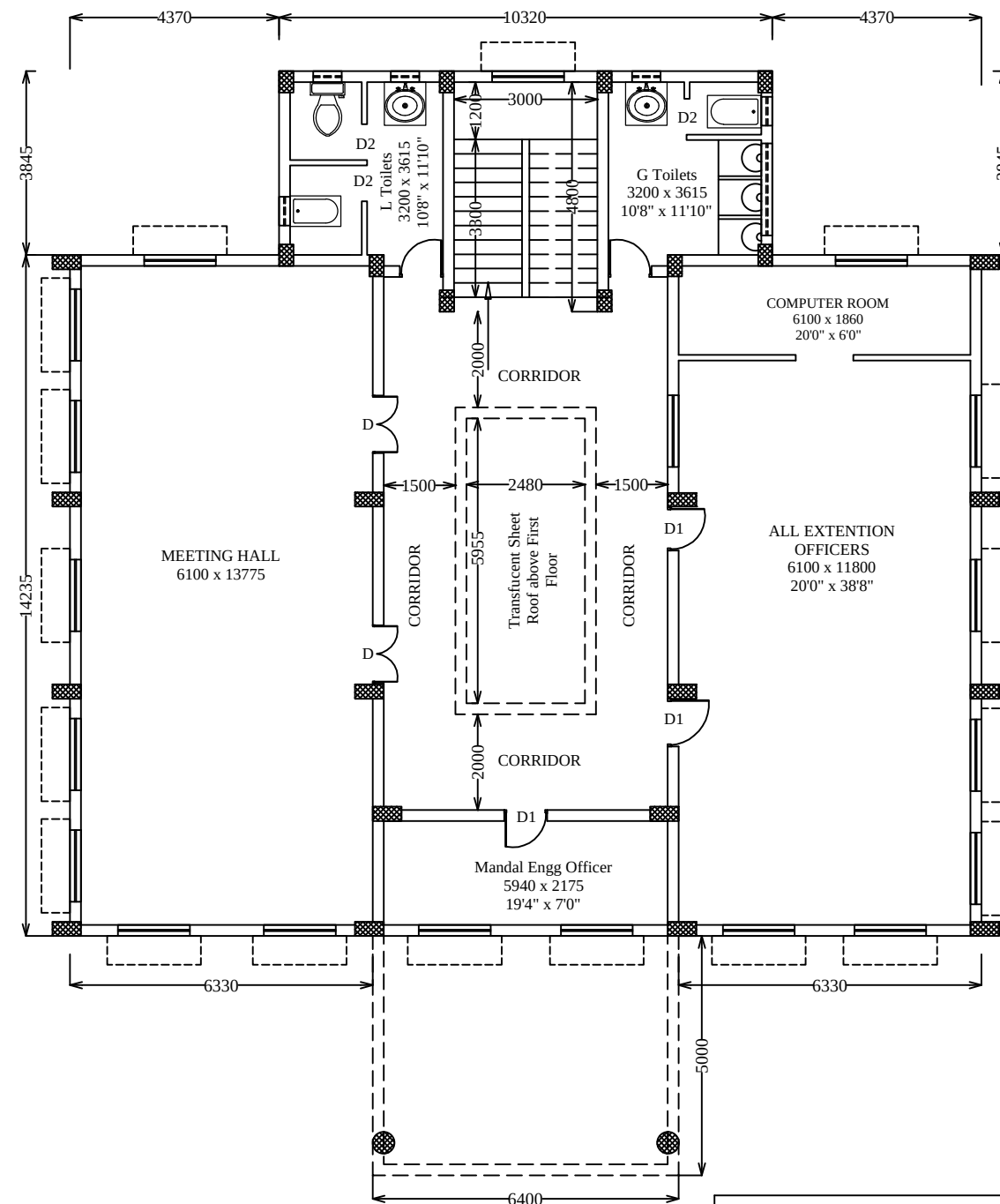
PROPOSED MPP OFFICE FIRST FLOOR PLAN
