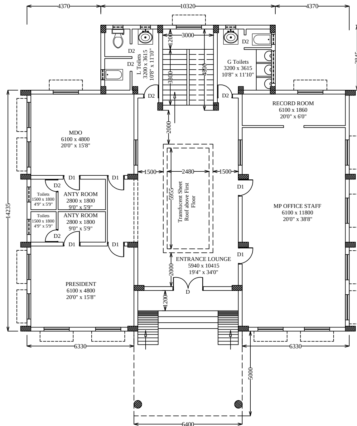
PROPOSED MPP OFFICE GROUND FLOOR PLAN
